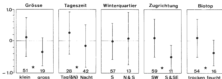
Abb. 2. Mittlere Abweichungen (Residuen) aus der in Abb. 1 dargestellten Beziehung für verschiedene Artengruppen (Einteilung s. Kap. 2.2.1.). Eingezeichnet ist der Mittelwert und die Standardabweichung. n = Anzahl Arten pro Gruppe (total jeweils 70). * = Unterschied zwischen den Gruppen signifikant (t-Test, s. Kap. 1.5.). – Mean residuals (from fig. 1) for various groups of species distinguished as follows: size (</> 50 g), time of migration (day/night), wintering area (south of the Alps to a considerable part north of the Alps), direction of migration in Europe (SW/S and SE), habitat (dependent/not dependent on wet habitats). Mean, standard deviation, number of species per group and asterisks for significant differences between groups are indicated.
